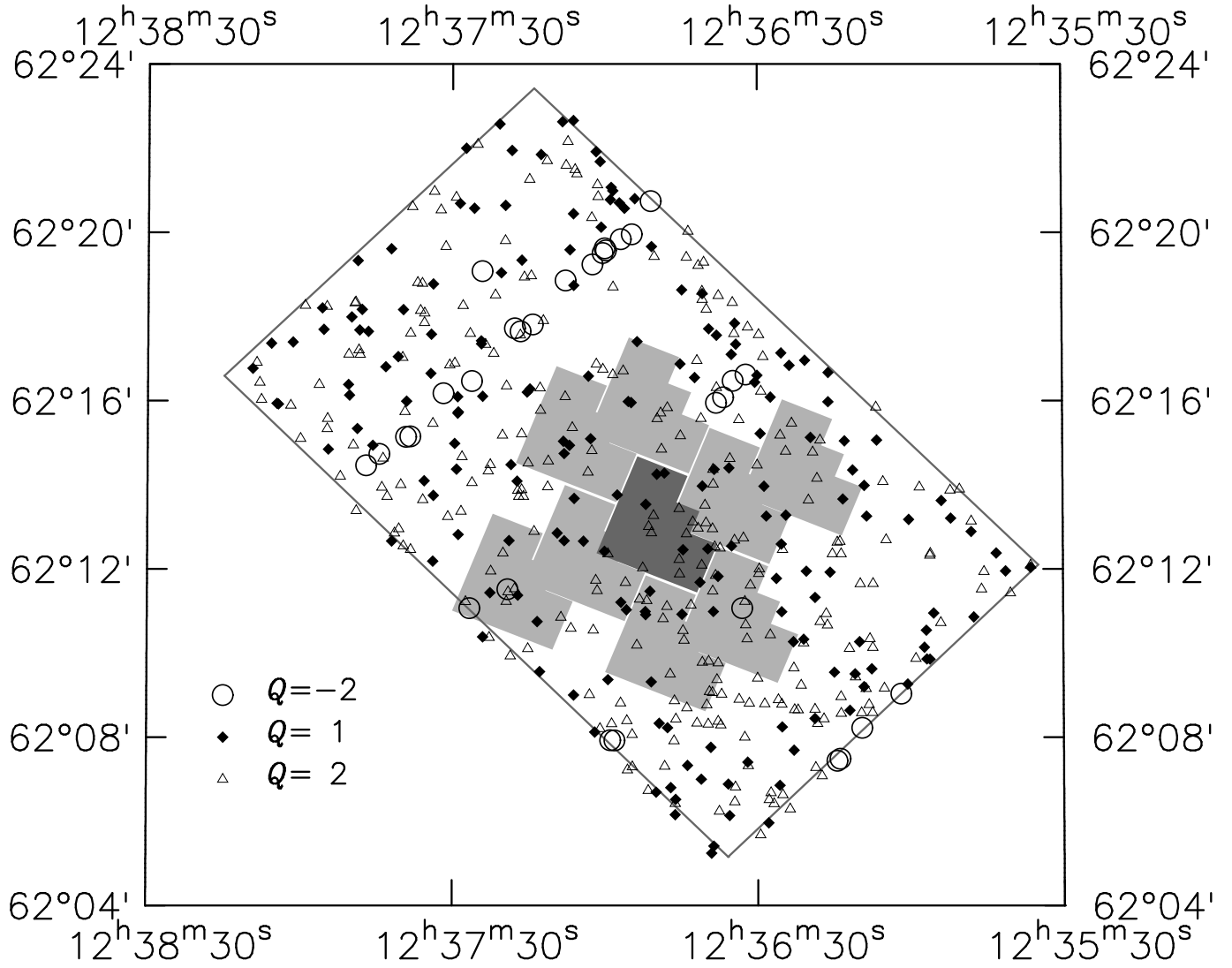
FIG. 6.— Projected sky distribution of objects for which no successful redshifts were measured. Plotting symbols distinguish objects for which no spectra were obtained because they fell on bad columns, gaps between CCDs, or at the edges of masks ( Q = -2 ), objects for which a spectrum was obtained, but no redshift could be deduced ( Q = 1 ), and objects which may yet produce redshifts or for which only one spectral feature was identified on the spectra ( Q = 2 ). Shaded regions indicate the HDF and flanking fields as in Fig. 3.
